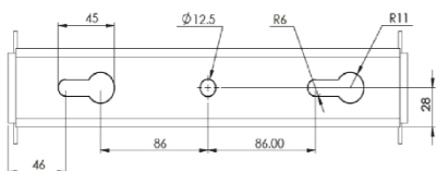
Bracket Top View
