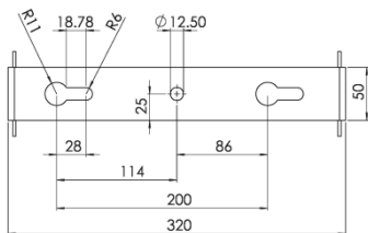
Bracket Top View
