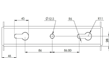
Bracket Top View
